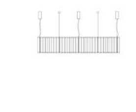
SM1318S-L1970/L1360 L1360×W240×H200 (MAX H2000) L1970×W310×H410 (MAX H2000)
